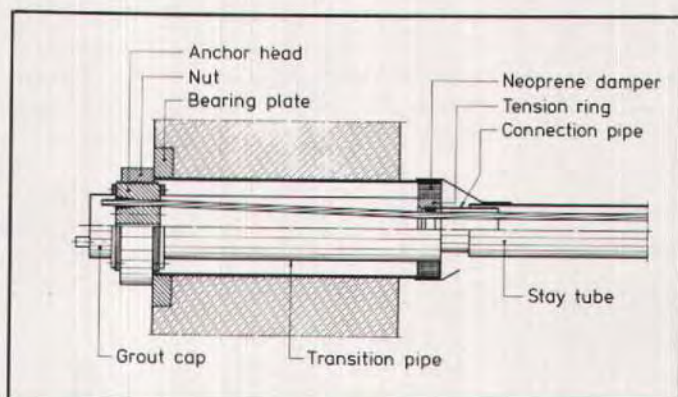
Fig. 36. VSL anchorage for strands.
