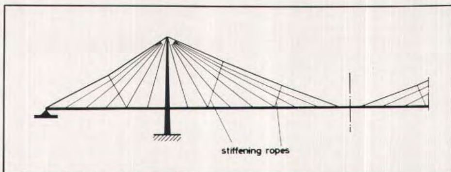
Fig. 6. Stiffening ropes afixed to long cables reduce cable sag.
