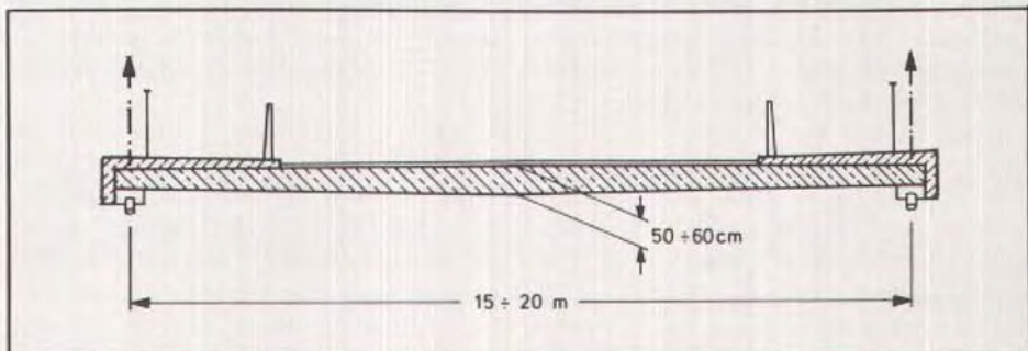
Fig. 24. Cross section with solid slab only for highway bridges with spans up to 150 m (490 ft).
